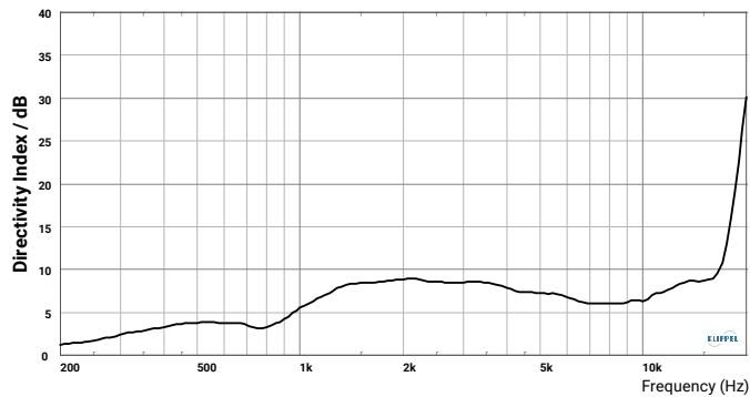
Directivity Index
