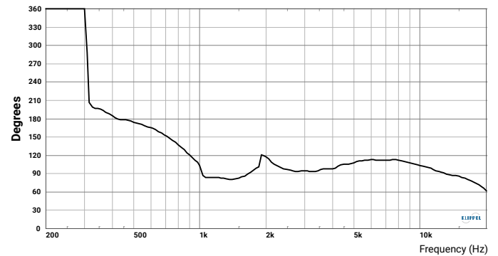
Vertical Beamwidth
