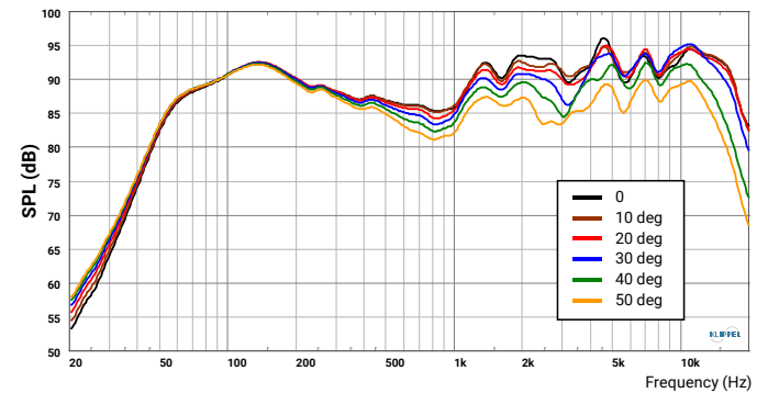
Frequency Response, Horizontal
