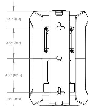
Rear View with bracket
