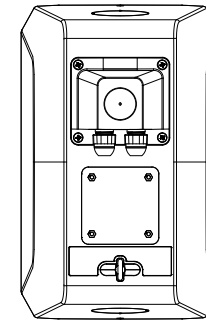
Rear View with terminal cover
