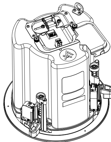
Isometric View (With connectors shown)
