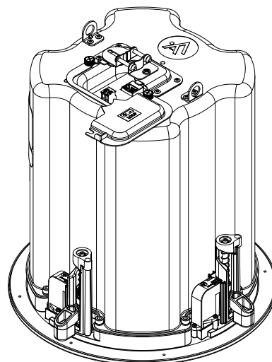
Isometric View (With connectors shown)
