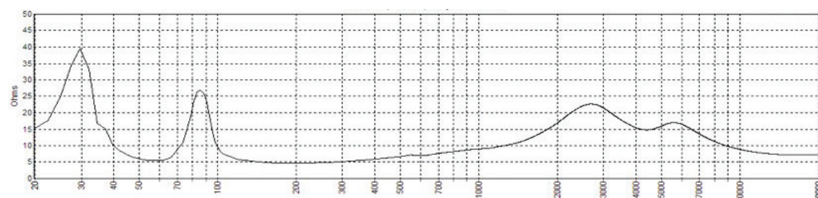
PM8CX Impedance
