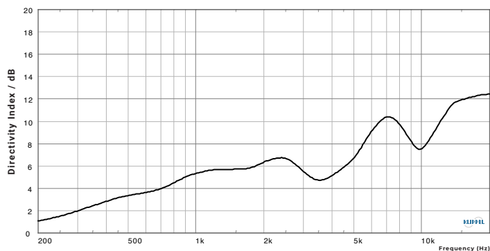
DIRECTIVITY INDEX
