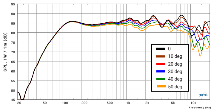
Frequency Response
