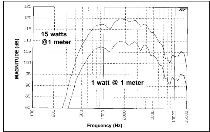
AP-15(T) Frequency Response
